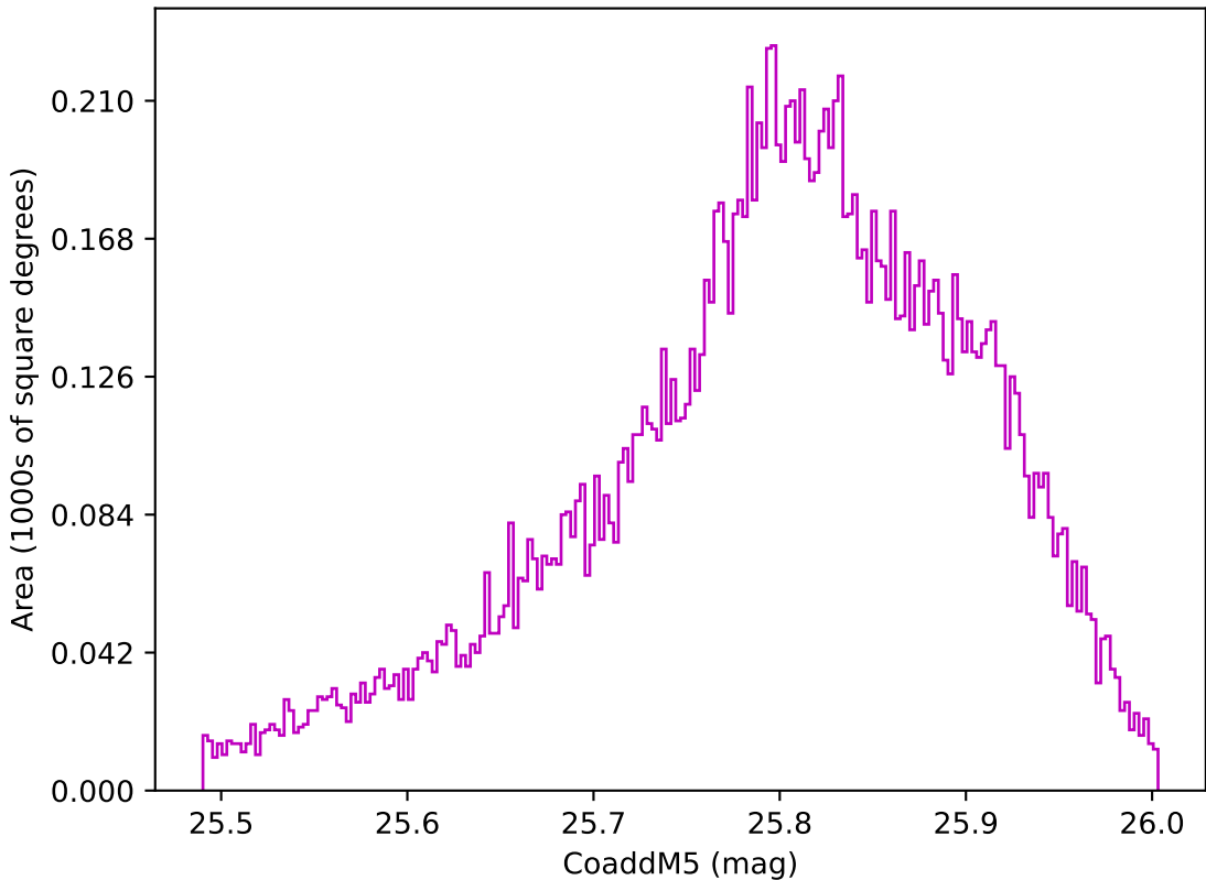
too_combined_no_nss_s10.0_v3.4_10yrs WFD z band: CoaddM5
