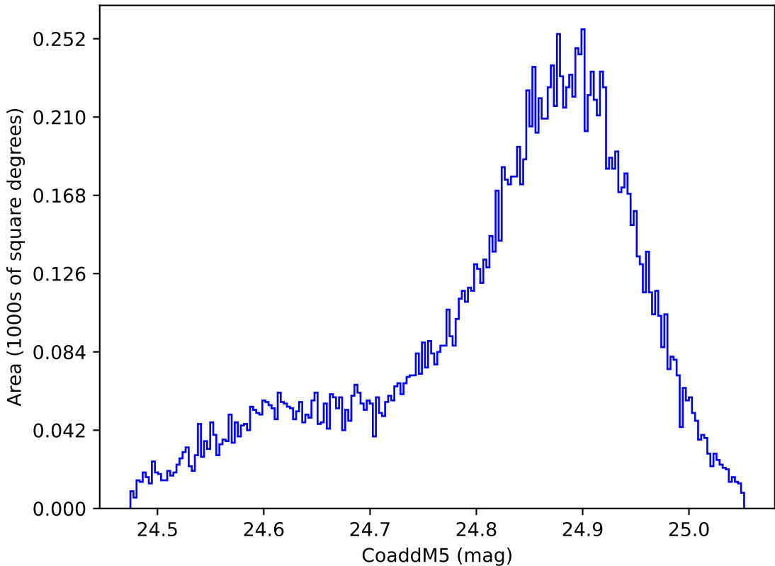
too_combined_no_nss_s10.0_v3.4_10yrs WFD y band: CoaddM5
