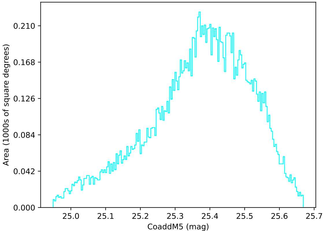
too_combined_no_nss_s10.0_v3.4_10yrs WFD u band: CoaddM5
