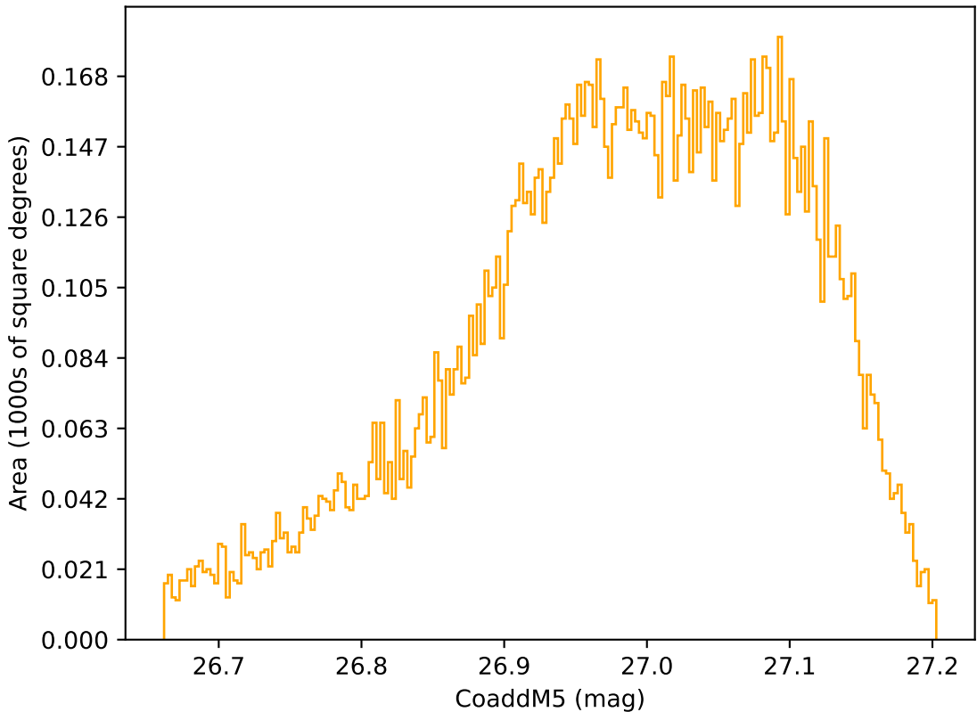
too_combined_no_nss_s10.0_v3.4_10yrs WFD r band: CoaddM5
