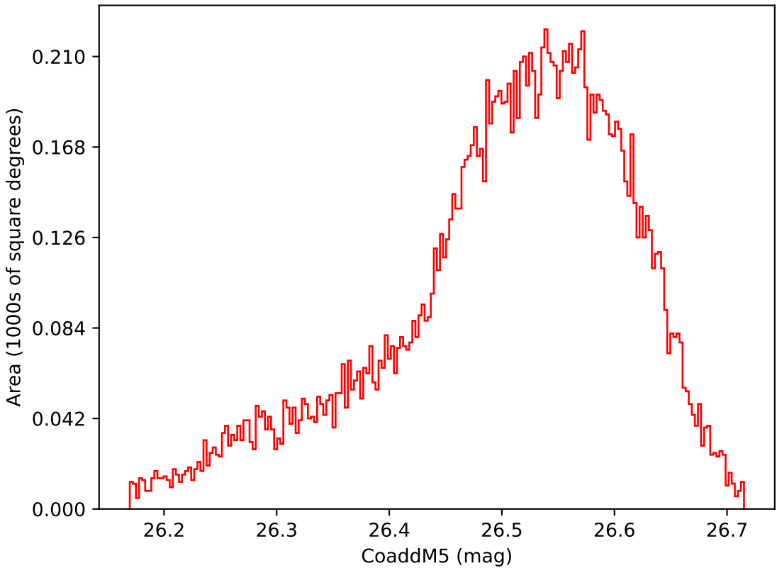
too_combined_no_nss_s10.0_v3.4_10yrs WFD i band: CoaddM5
