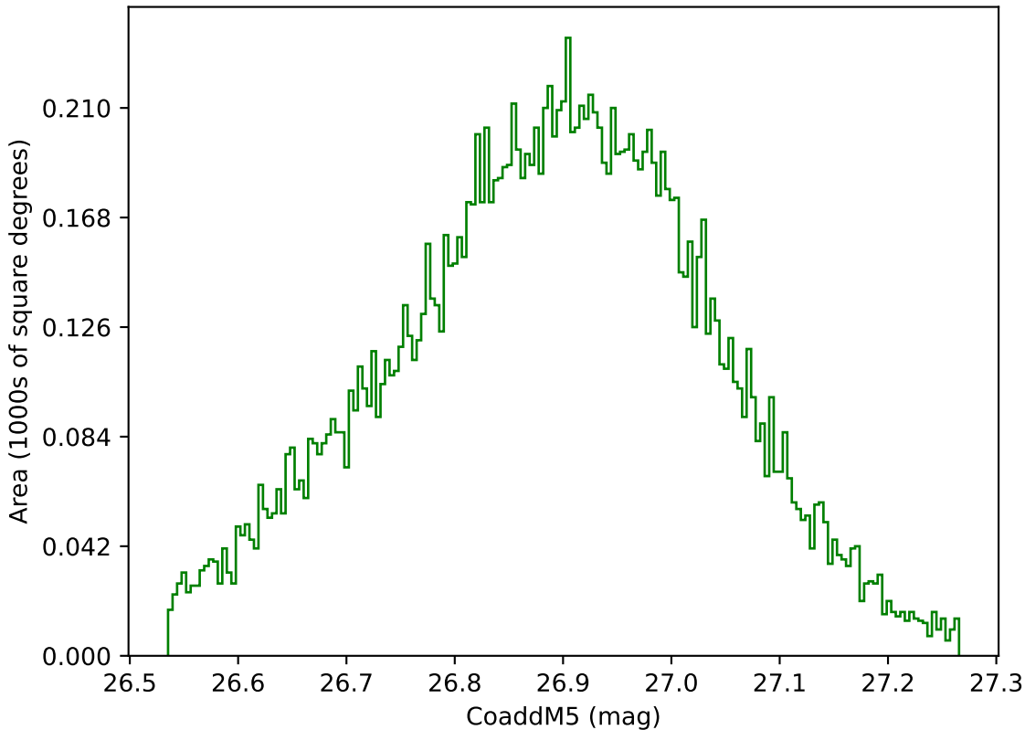
too_combined_no_nss_s10.0_v3.4_10yrs WFD g band: CoaddM5
