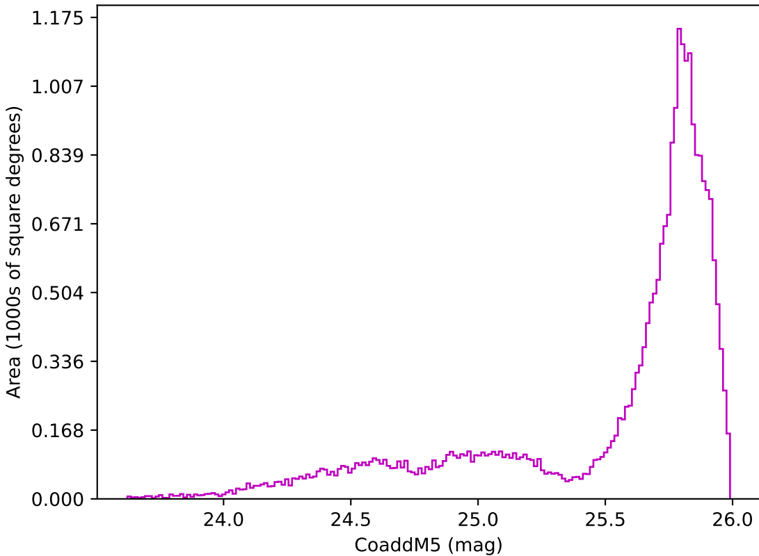
too_combined_no_nss_s10.0_v3.4_10yrs All sky z band: CoaddM5
