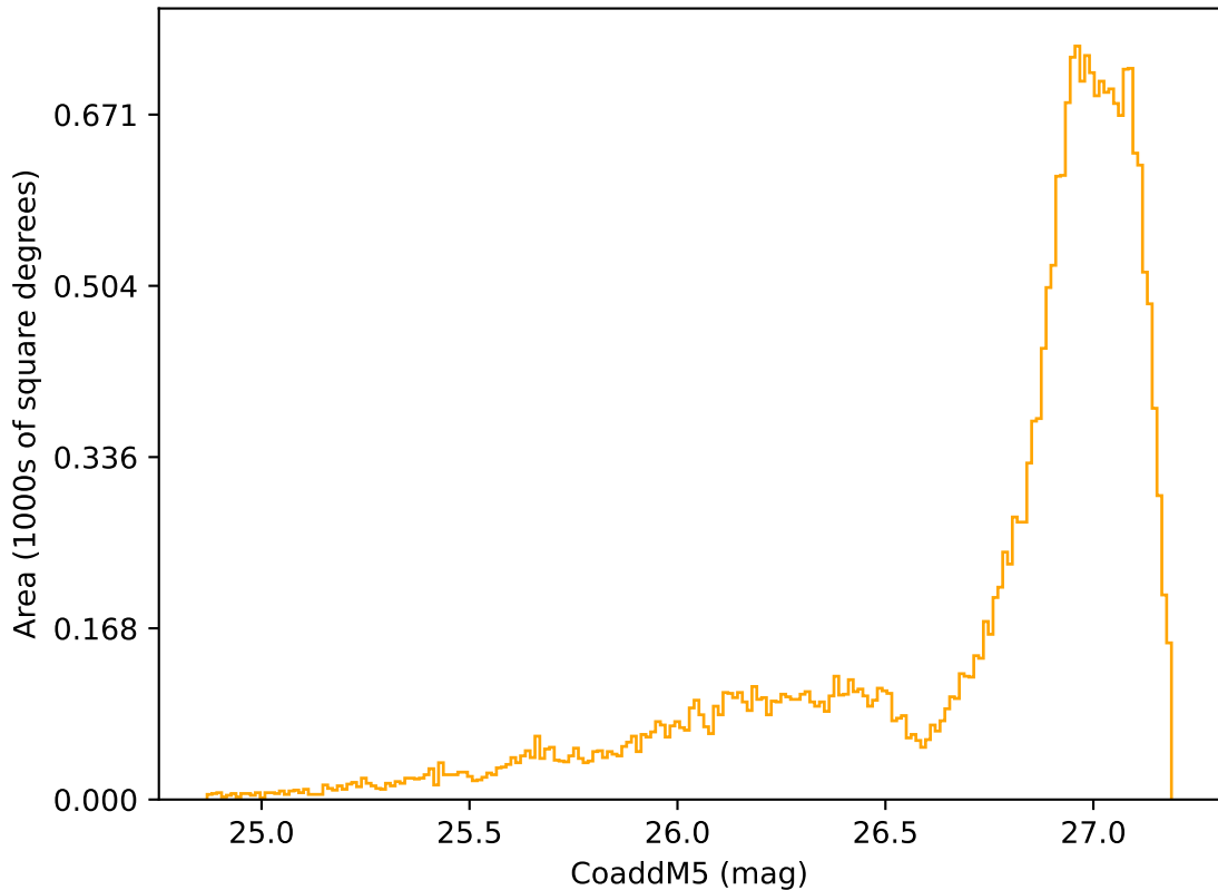
too_combined_no_nss_s10.0_v3.4_10yrs All sky r band: CoaddM5
