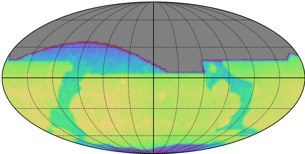
too_combined_no_nss_s10.0_v3.4_10yrs All sky i band: CoaddM5
