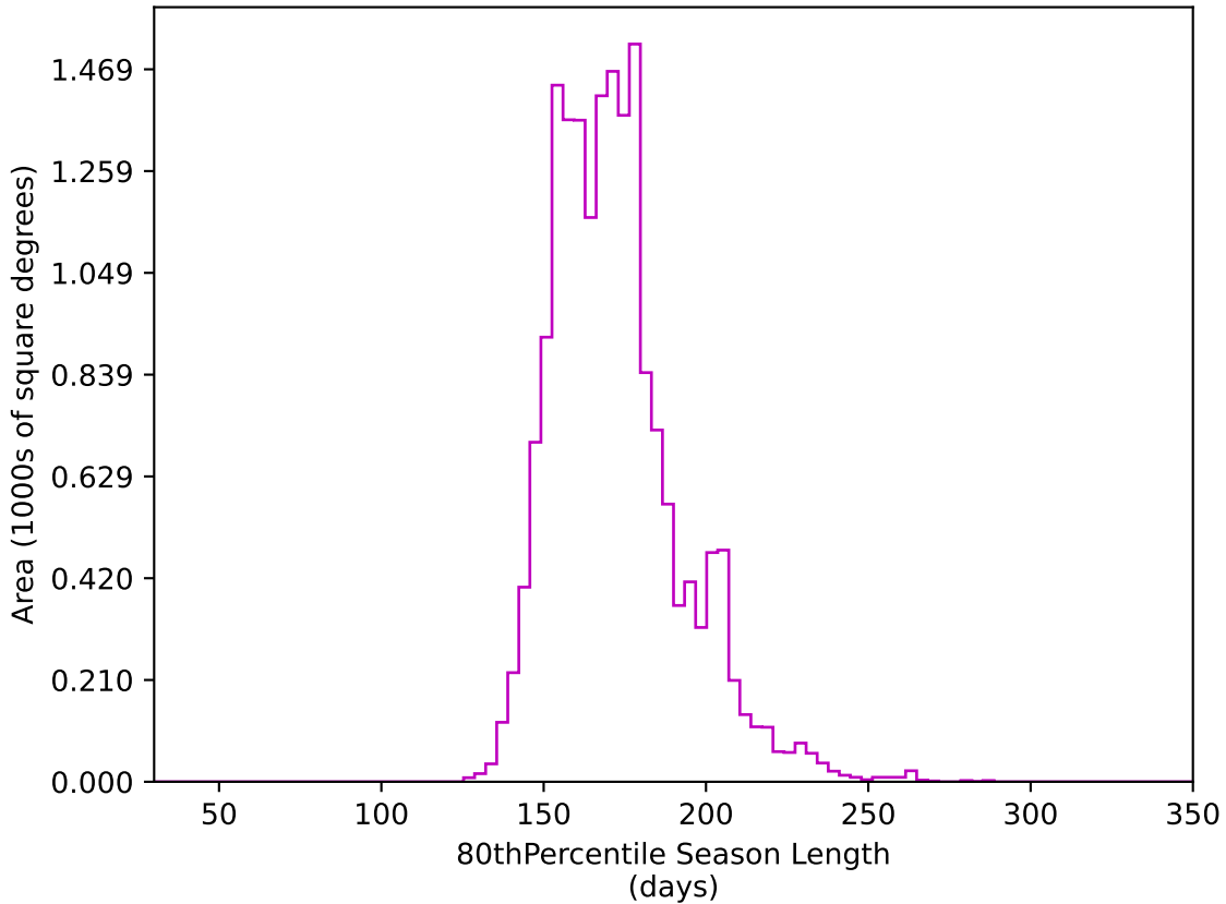
too_combined_no_nss_s10.0_v3.4_10yrs WFD z band: 80thPercentile Season Length
