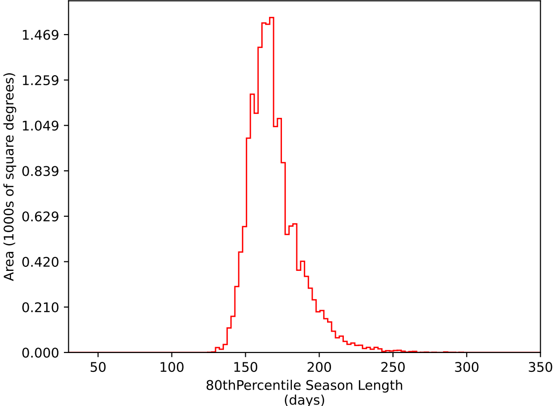
too_combined_no_nss_s10.0_v3.4_10yrs WFD i band: 80thPercentile Season Length
