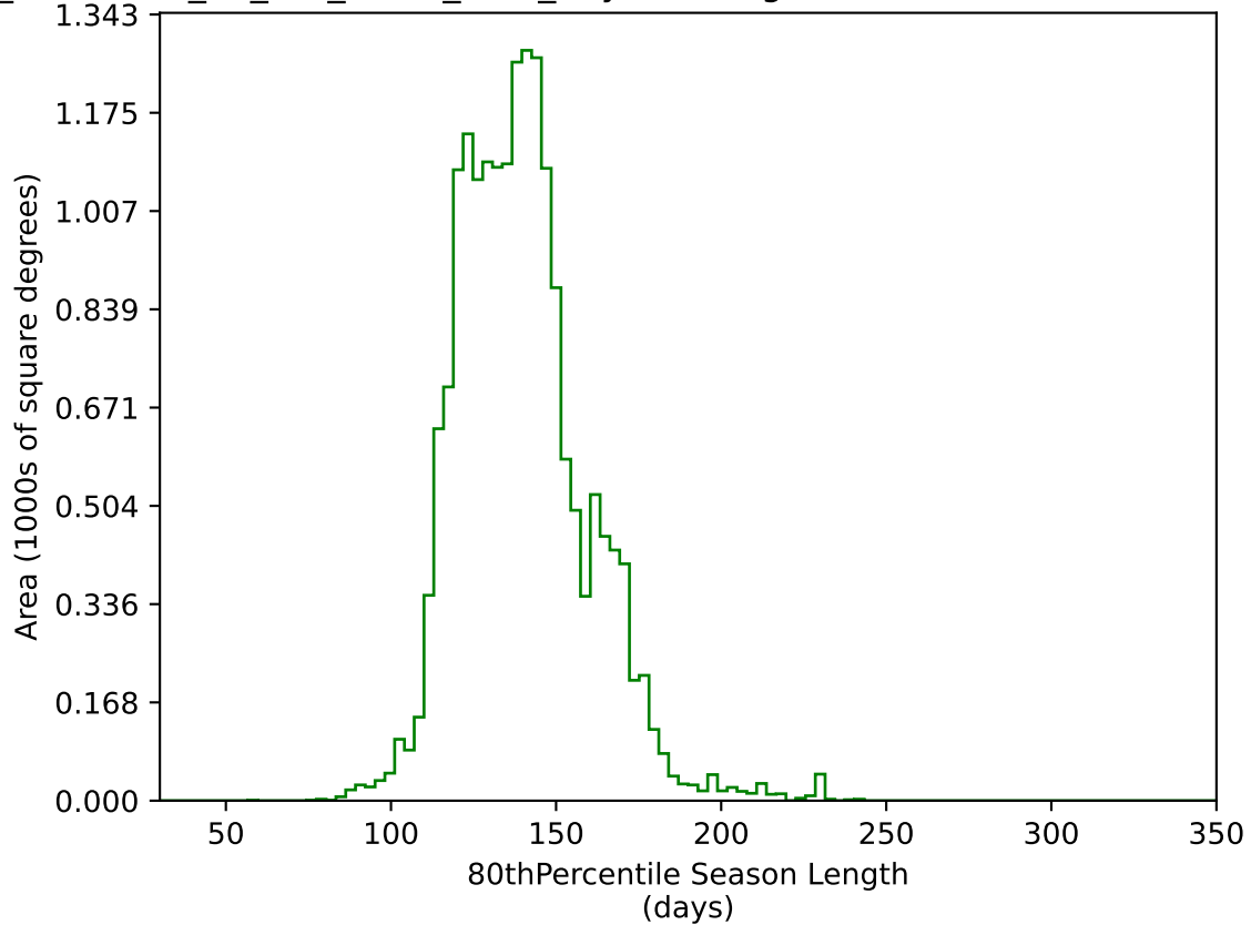
too_combined_no_nss_s10.0_v3.4_10yrs WFD g band: 80thPercentile Season Length
