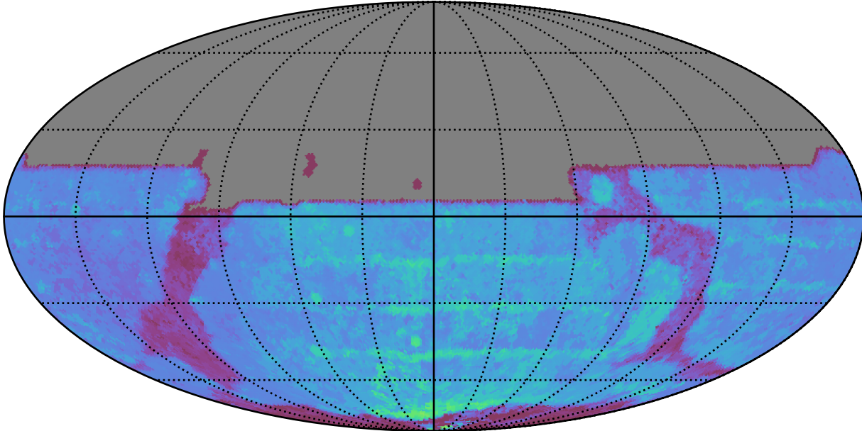
too_combined_no_nss_s10.0_v3.4_10yrs All sky y band: 80thPercentile Season Length
