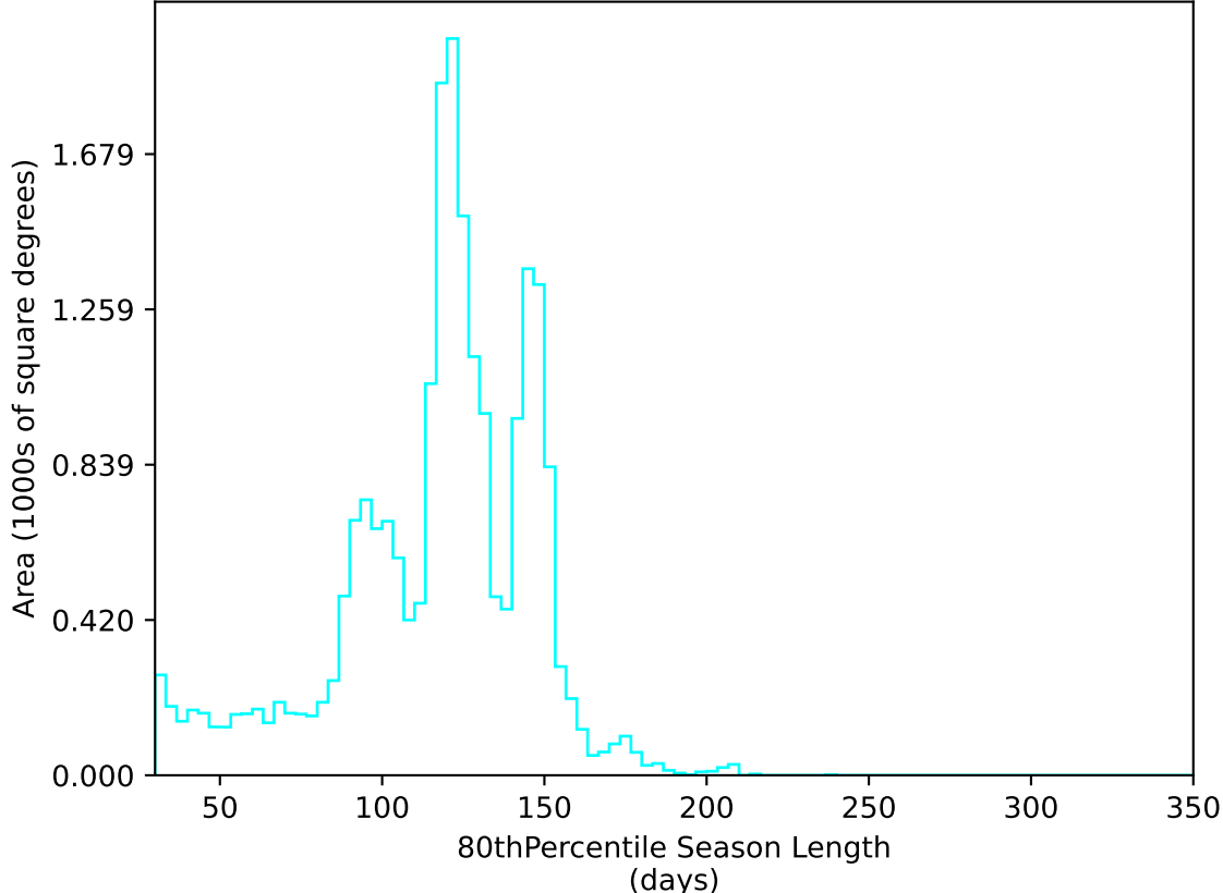
too_combined_no_nss_s10.0_v3.4_10yrs All sky u band: 80thPercentile Season Length
