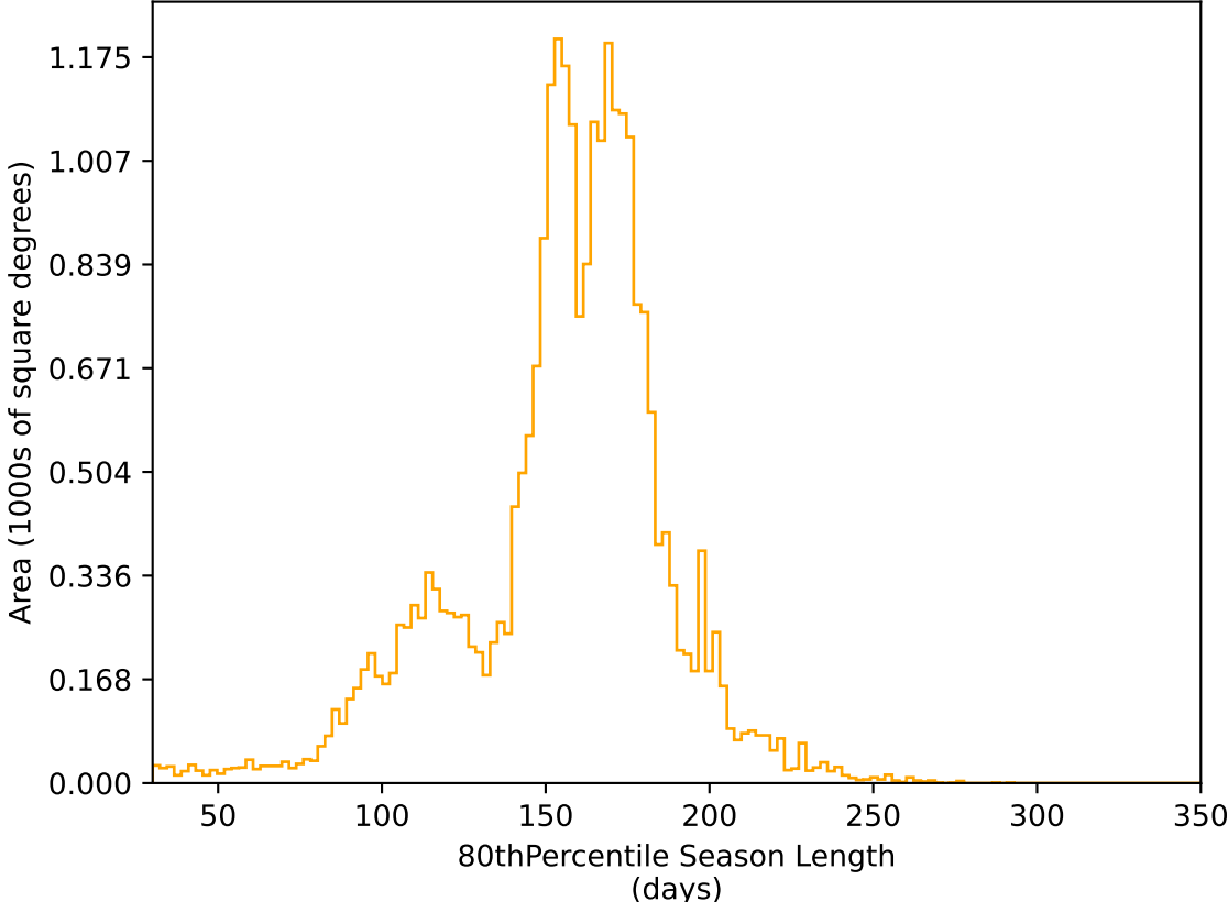
too_combined_no_nss_s10.0_v3.4_10yrs All sky r band: 80thPercentile Season Length
