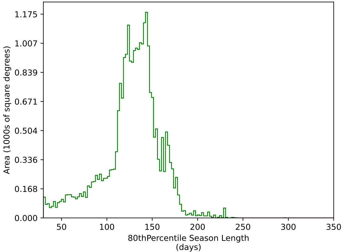
too_combined_no_nss_s10.0_v3.4_10yrs All sky g band: 80thPercentile Season Length
