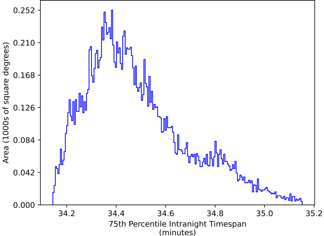
too_combined_no_nss_s10.0_v3.4_10yrs WFD zy bands: 75th Percentile Intranight Timespan
