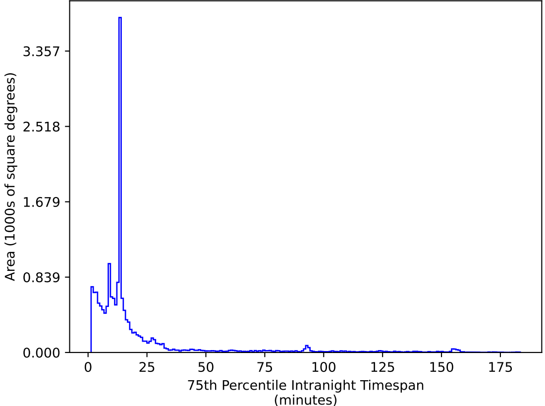
too_combined_no_nss_s10.0_v3.4_10yrs WFD z band: 75th Percentile Intranight Timespan
