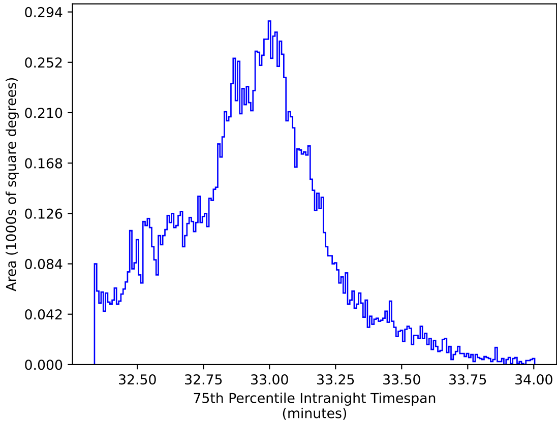
too_combined_no_nss_s10.0_v3.4_10yrs WFD y band: 75th Percentile Intranight Timespan
