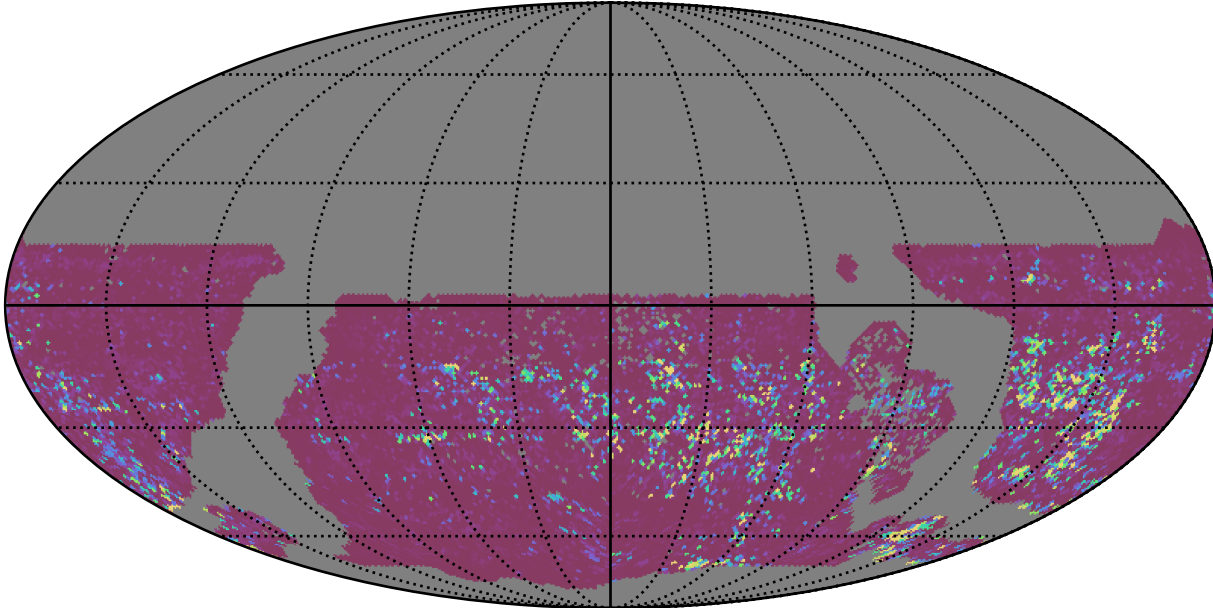
too_combined_no_nss_s10.0_v3.4_10yrs WFD u band: 75th Percentile Intranight Timespan
