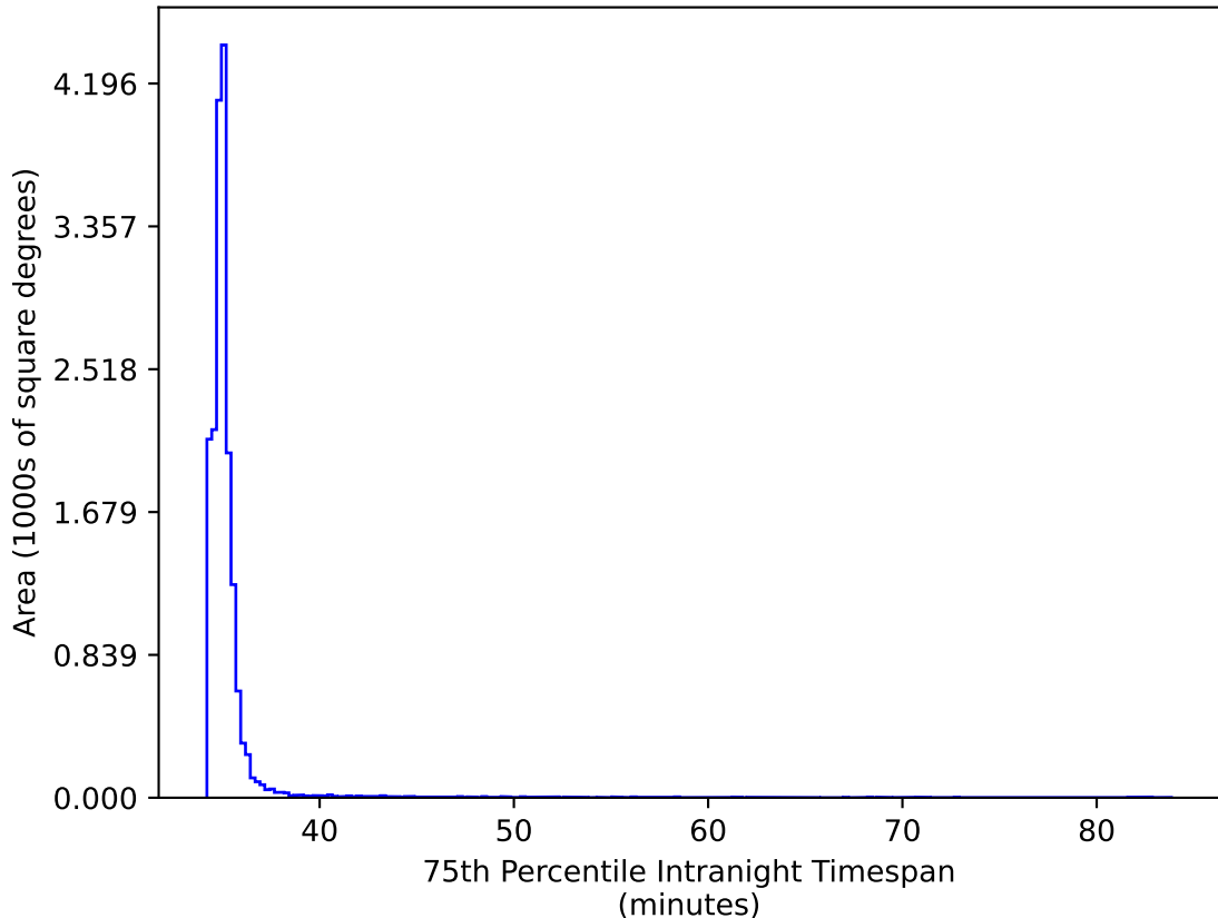
too_combined_no_nss_s10.0_v3.4_10yrs WFD ri bands: 75th Percentile Intranight Timespan
