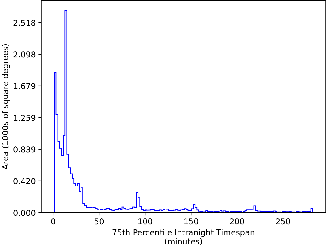
too_combined_no_nss_s10.0_v3.4_10yrs WFD r band: 75th Percentile Intranight Timespan
