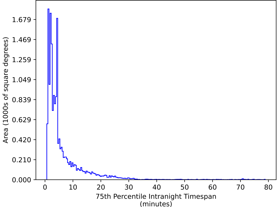
too_combined_no_nss_s10.0_v3.4_10yrs WFD g band: 75th Percentile Intranight Timespan
