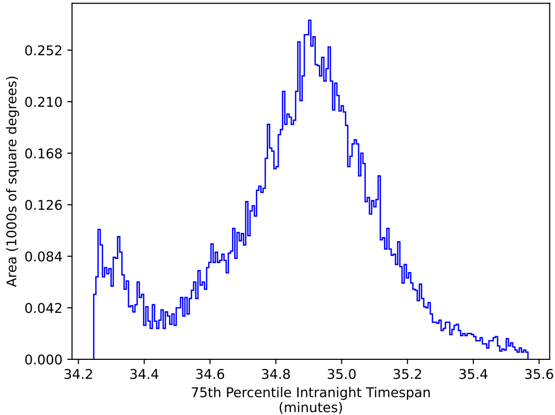
too_combined_no_nss_s10.0_v3.4_10yrs WFD: 75th Percentile Intranight Timespan
