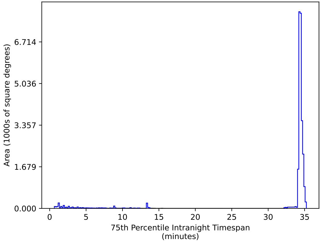
too_combined_no_nss_s10.0_v3.4_10yrs All sky zy bands: 75th Percentile Intranight Timespan
