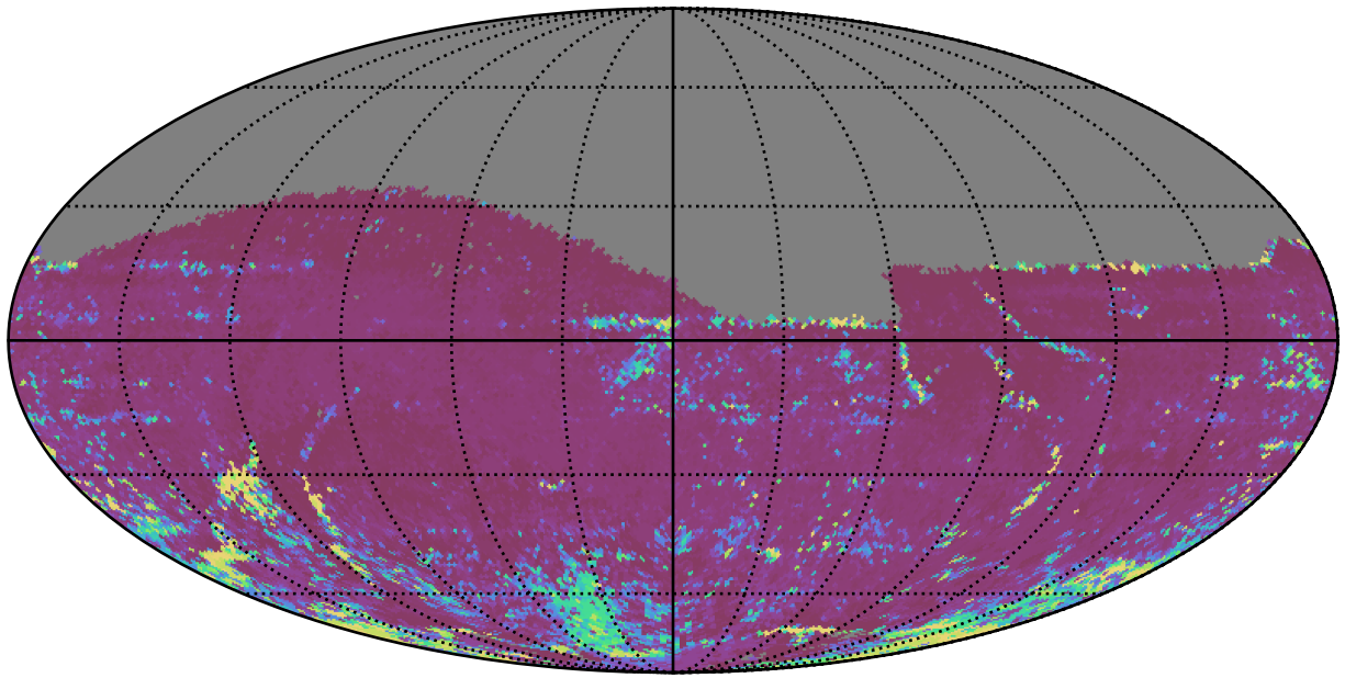
too_combined_no_nss_s10.0_v3.4_10yrs All sky z band: 75th Percentile Intranight Timespan
