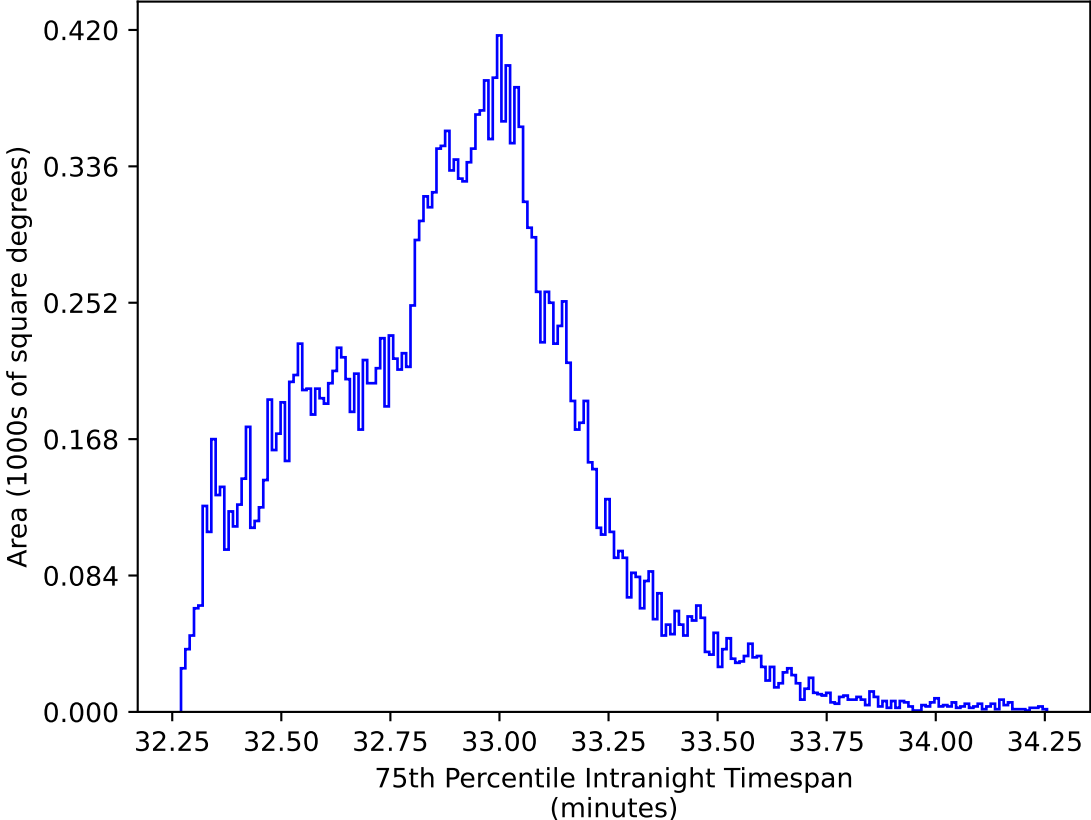
too_combined_no_nss_s10.0_v3.4_10yrs All sky y band: 75th Percentile Intranight Timespan
