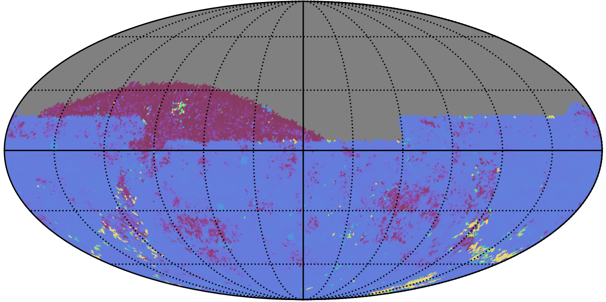
too_combined_no_nss_s10.0_v3.4_10yrs All sky ug bands: 75th Percentile Intranight Timespan
