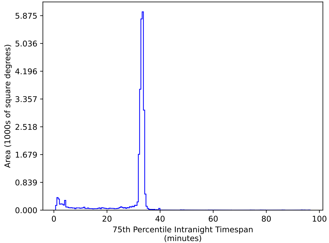
too_combined_no_nss_s10.0_v3.4_10yrs All sky ug bands: 75th Percentile Intranight Timespan
