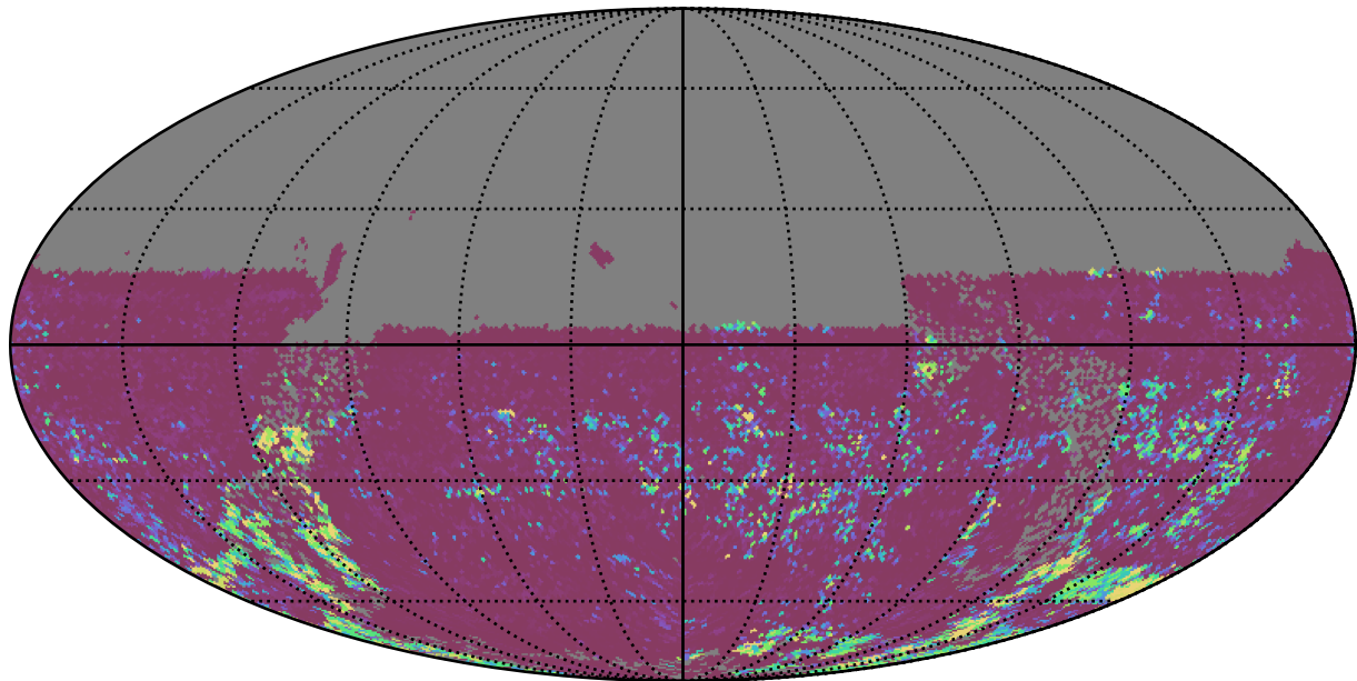
too_combined_no_nss_s10.0_v3.4_10yrs All sky u band: 75th Percentile Intranight Timespan
