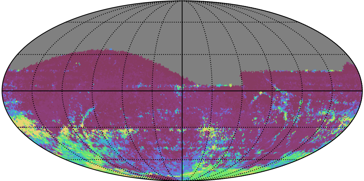
too_combined_no_nss_s10.0_v3.4_10yrs All sky r band: 75th Percentile Intranight Timespan
