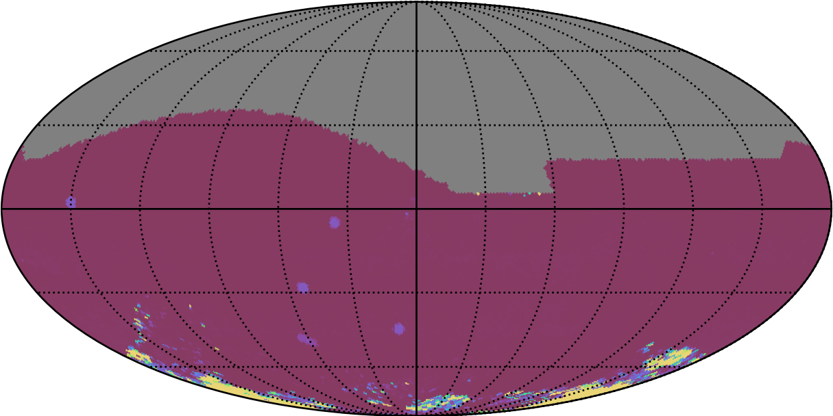
too_combined_no_nss_s10.0_v3.4_10yrs All sky iz bands: 75th Percentile Intranight Timespan
