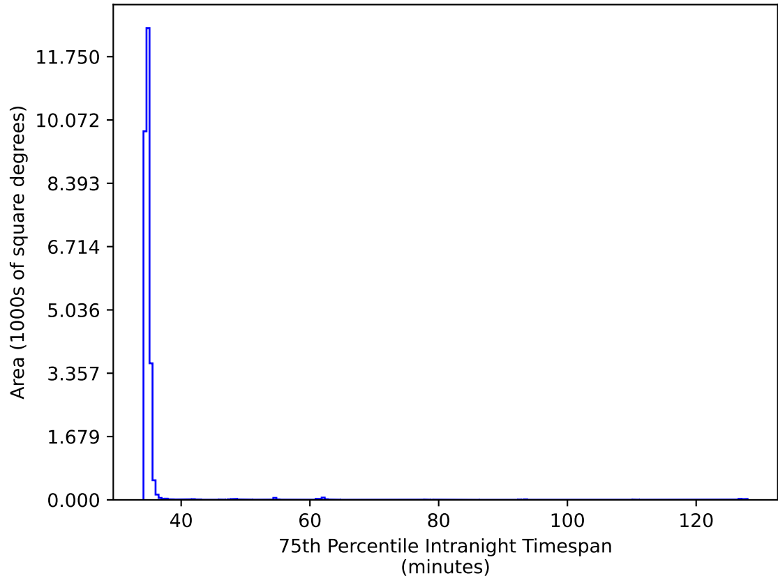
too_combined_no_nss_s10.0_v3.4_10yrs All sky iz bands: 75th Percentile Intranight Timespan
