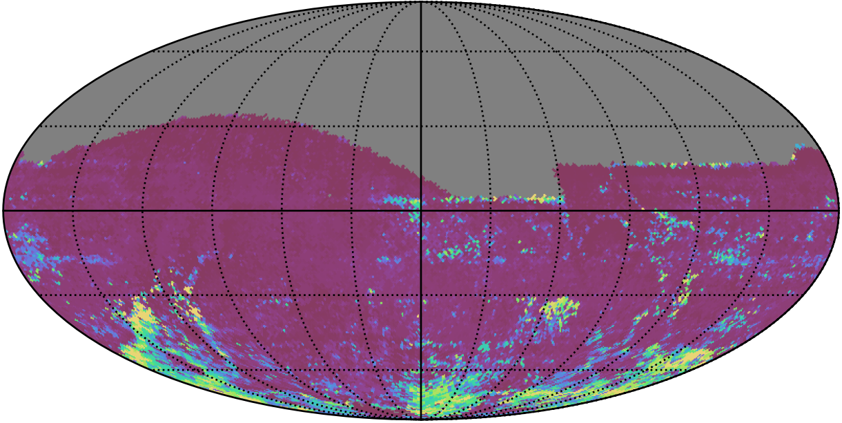
too_combined_no_nss_s10.0_v3.4_10yrs All sky i band: 75th Percentile Intranight Timespan
