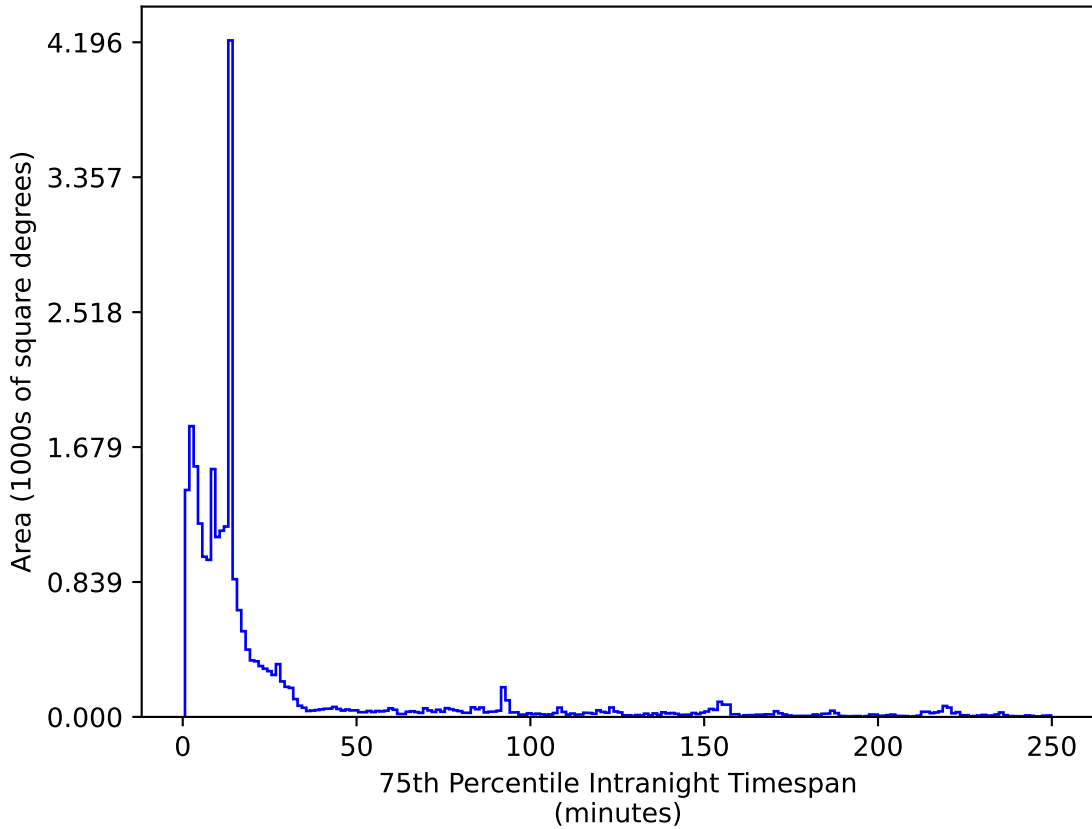
too_combined_no_nss_s10.0_v3.4_10yrs All sky i band: 75th Percentile Intranight Timespan
