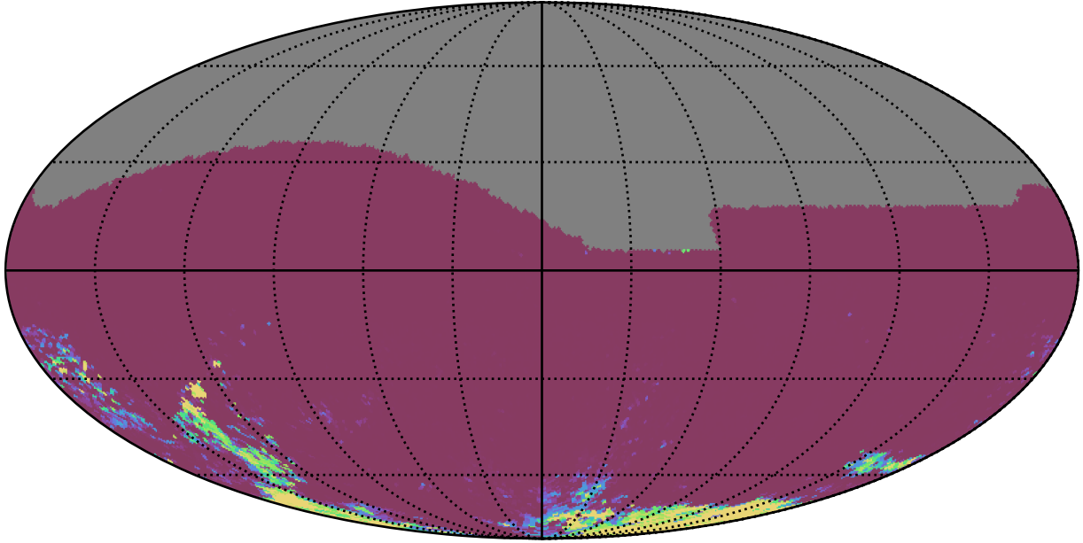
too_combined_no_nss_s10.0_v3.4_10yrs All sky gr bands: 75th Percentile Intranight Timespan
