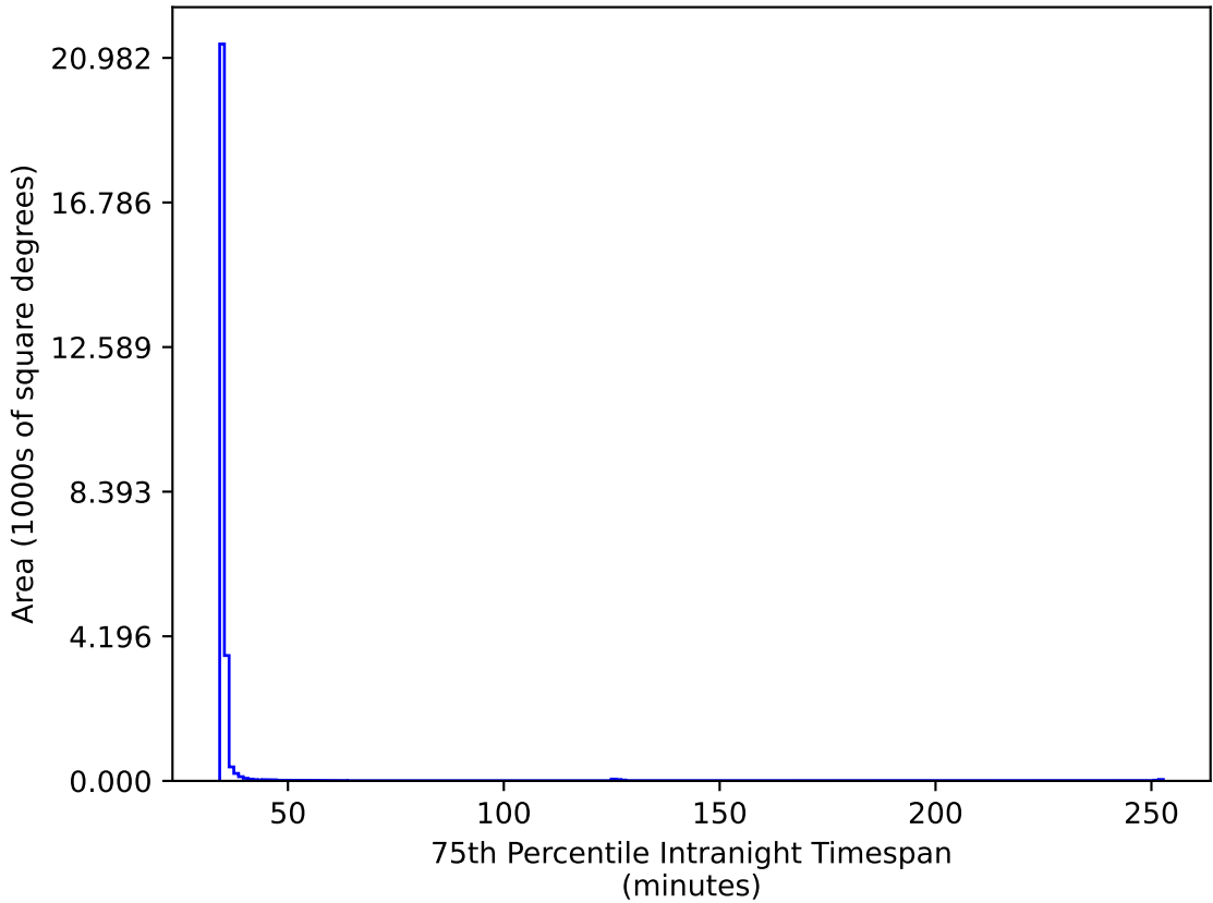
too_combined_no_nss_s10.0_v3.4_10yrs All sky gr bands: 75th Percentile Intranight Timespan
