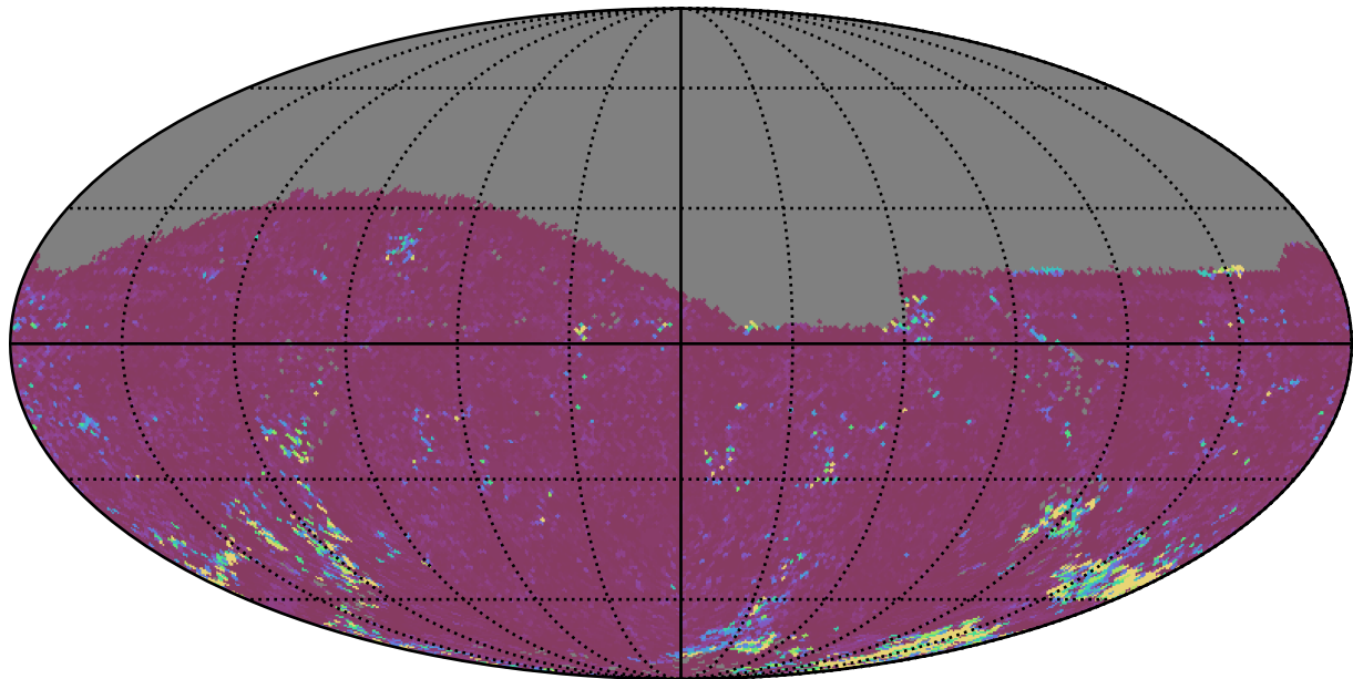
too_combined_no_nss_s10.0_v3.4_10yrs All sky g band: 75th Percentile Intranight Timespan
