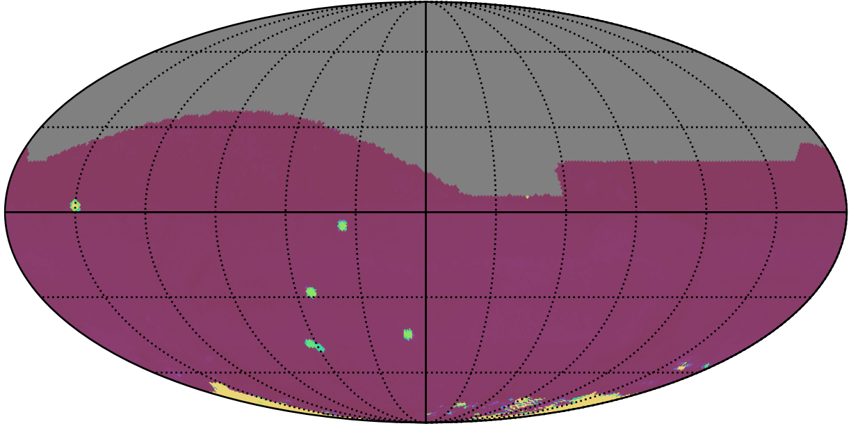
too_combined_no_nss_s10.0_v3.4_10yrs All sky all bands: 75th Percentile Intranight Timespan
