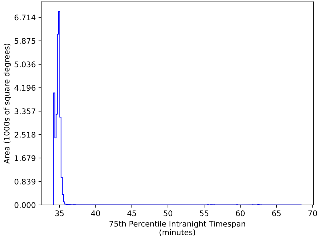
too_combined_no_nss_s10.0_v3.4_10yrs All sky all bands: 75th Percentile Intranight Timespan
