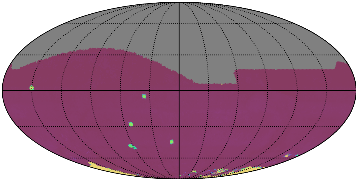
too_combined_no_nss_s10.0_v3.4_10yrs All sky: 75th Percentile Intranight Timespan
