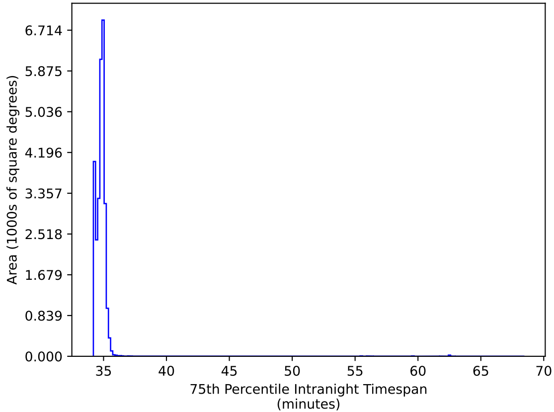
too_combined_no_nss_s10.0_v3.4_10yrs All sky: 75th Percentile Intranight Timespan
