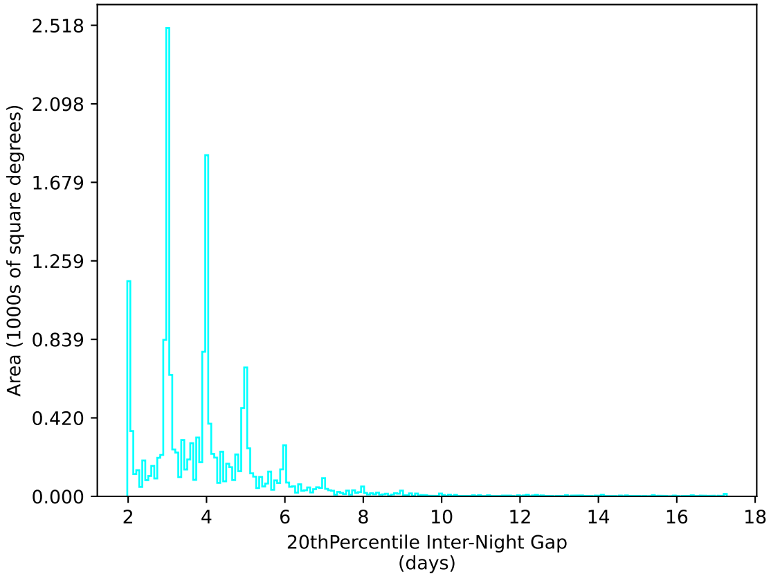
too_combined_no_nss_s10.0_v3.4_10yrs WFD u band: 20thPercentile Inter-Night Gap
