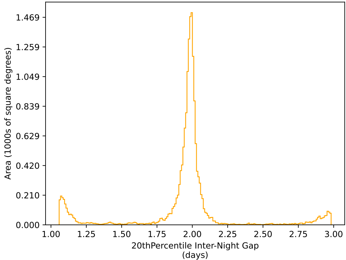
too_combined_no_nss_s10.0_v3.4_10yrs WFD r band: 20thPercentile Inter-Night Gap
