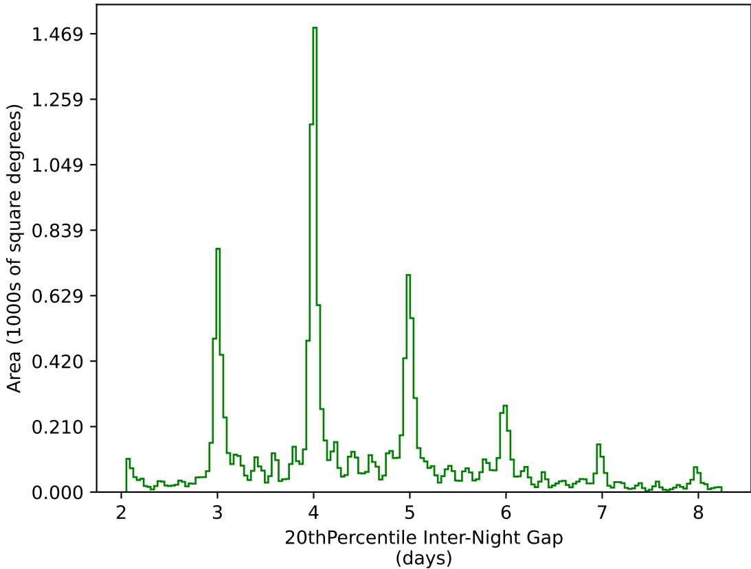
too_combined_no_nss_s10.0_v3.4_10yrs WFD g band: 20thPercentile Inter-Night Gap
