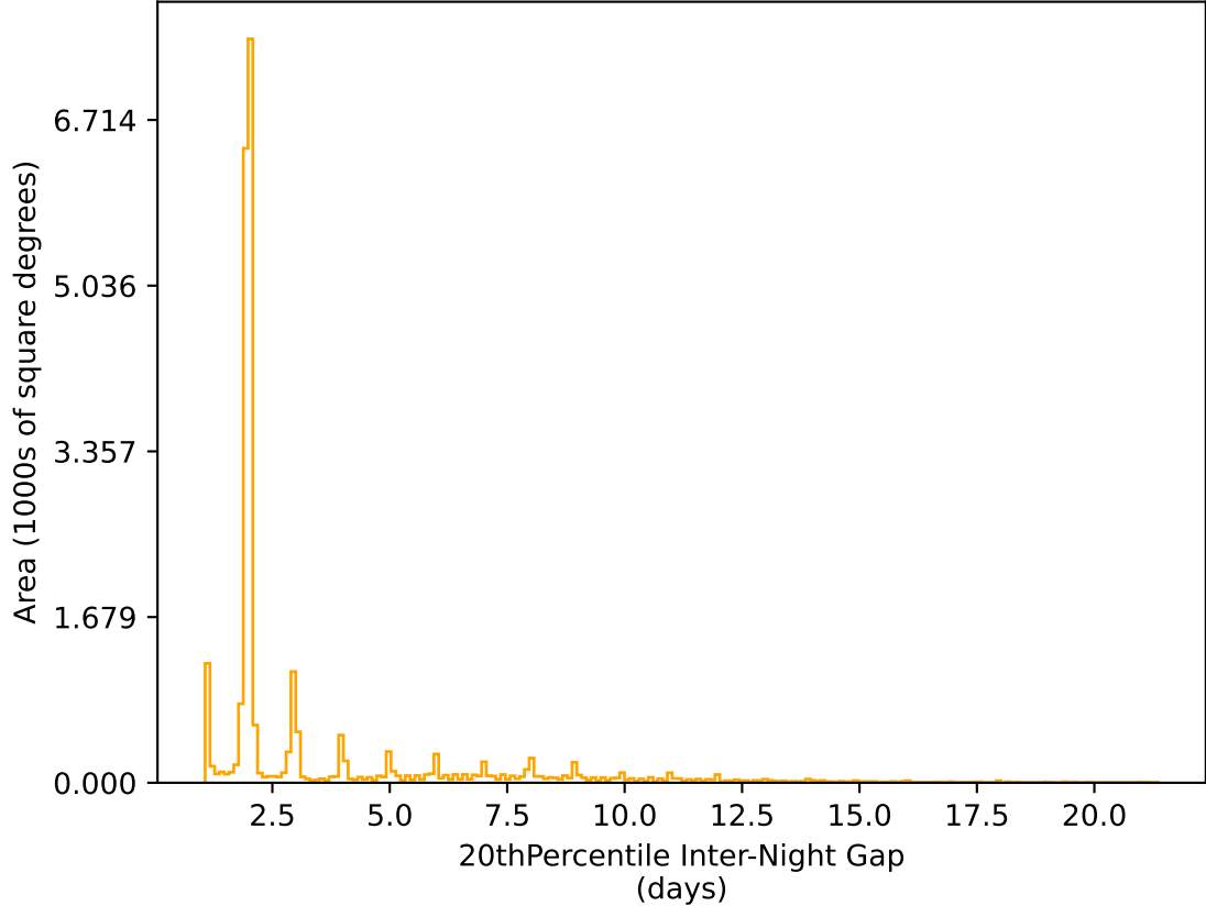
too_combined_no_nss_s10.0_v3.4_10yrs All sky r band: 20thPercentile Inter-Night Gap
