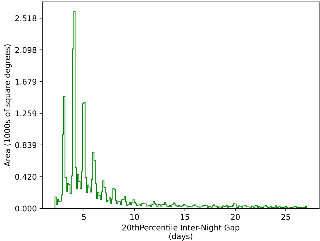
too_combined_no_nss_s10.0_v3.4_10yrs All sky g band: 20thPercentile Inter-Night Gap
