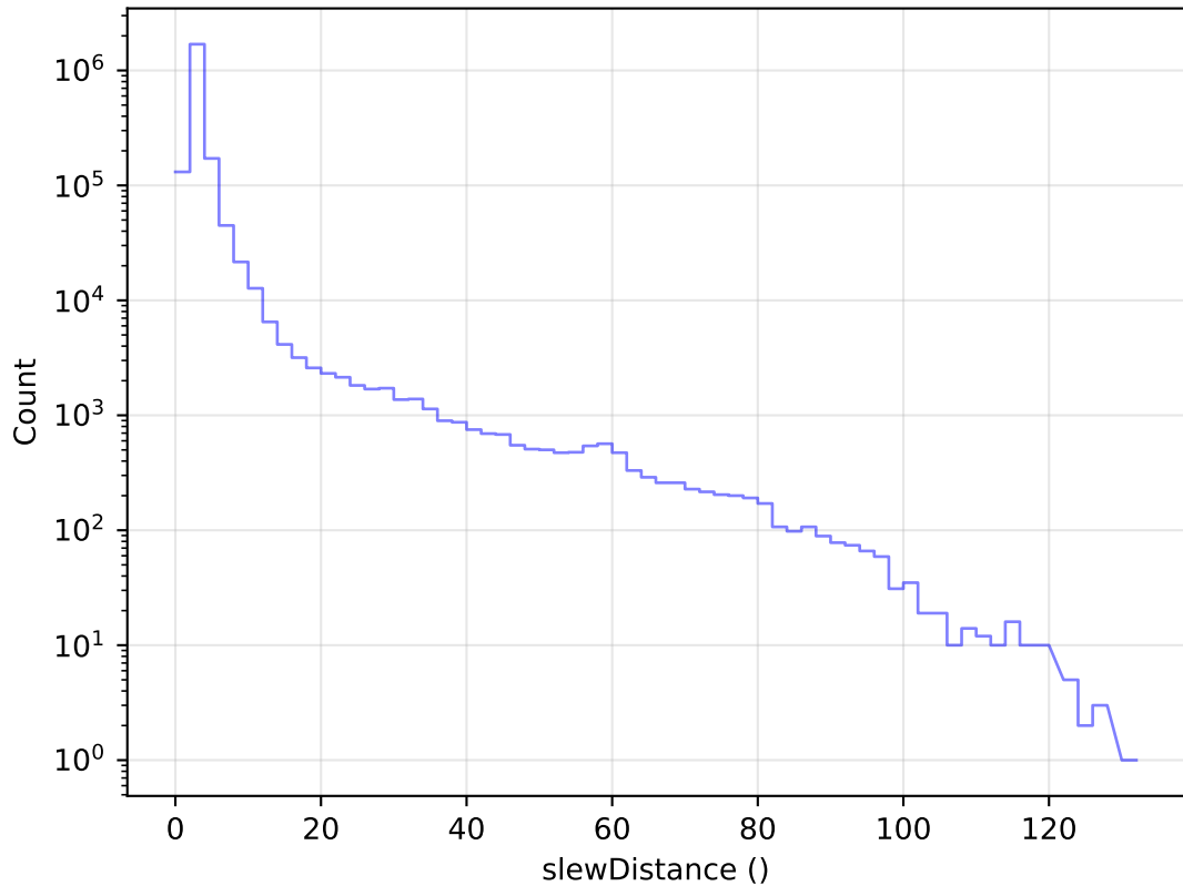
too_combined_no_nss_s10.0_v3.4_10yrs All visits: Slew Distance Histogram
