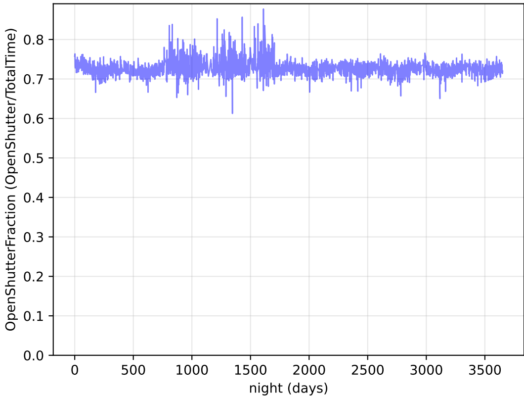
too_combined_no_nss_s10.0_v3.4_10yrs : OpenShutterFraction
