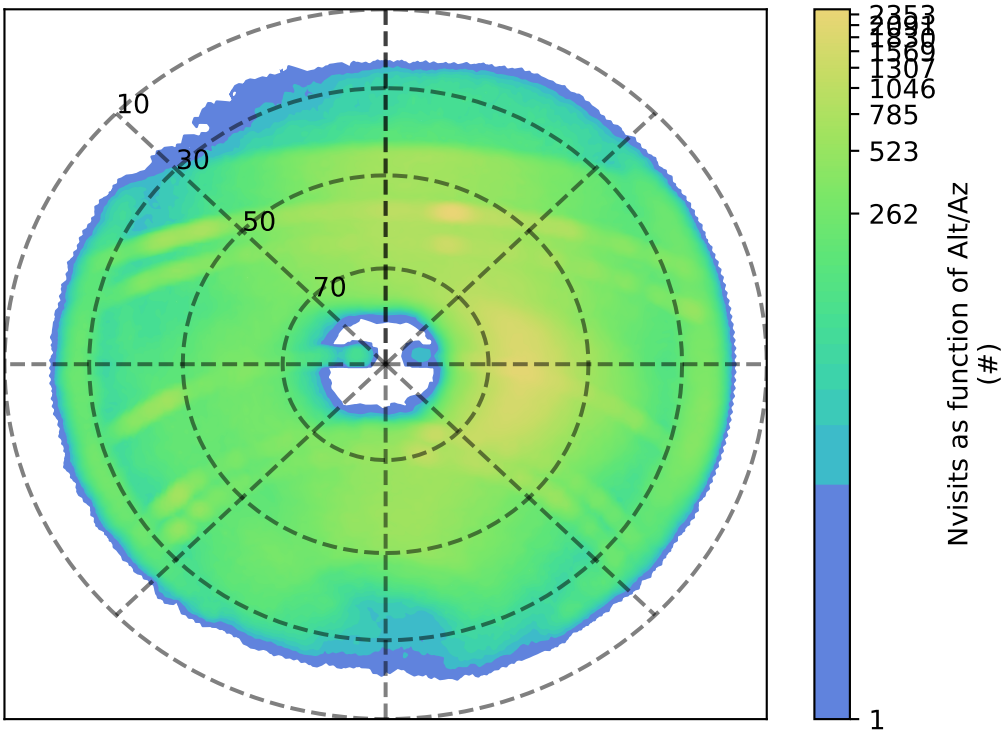
too_combined_no_nss_s10.0_v3.4_10yrs z: Nvisits as function of Alt/Az
